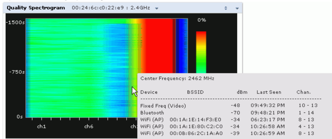
Figure 147 Quality Spectrogram
