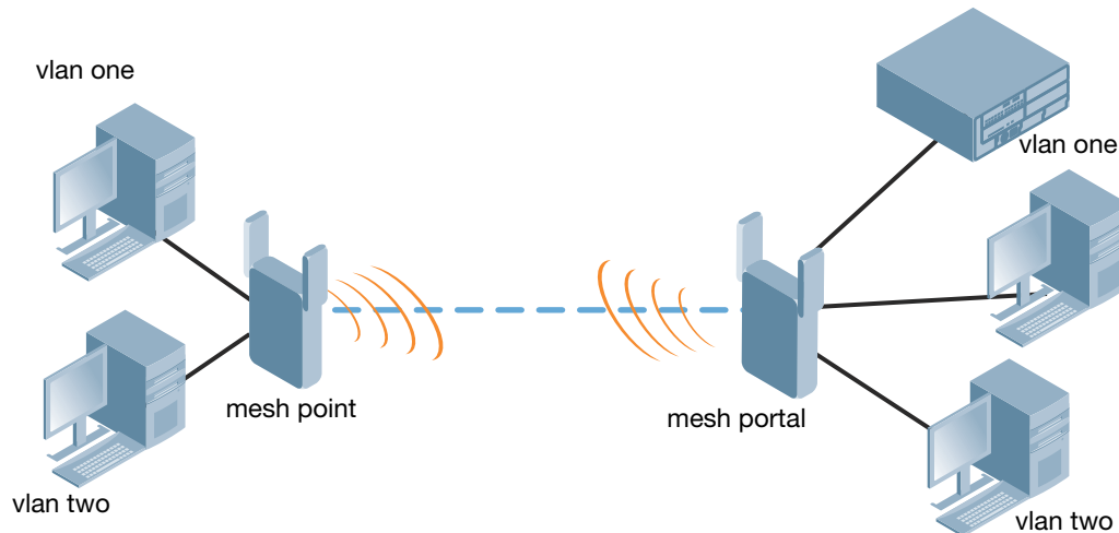
Figure 36 Sample Point-to-Point Deployment
