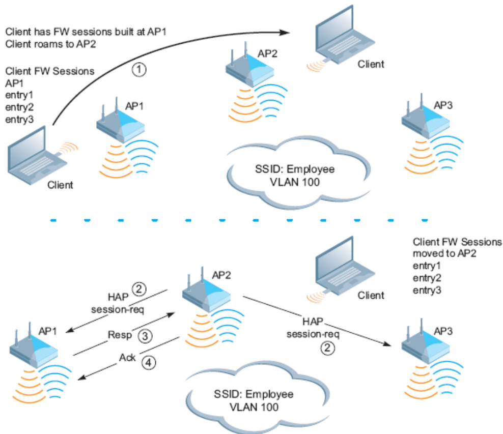
Figure 75 Bridge Mode Mobility
