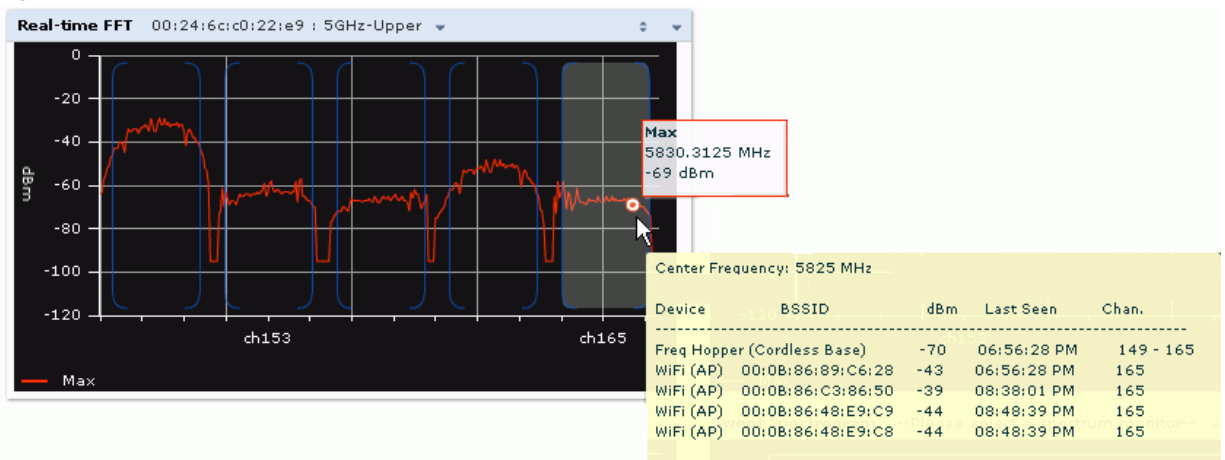
Figure 148 Real-Time FFT
