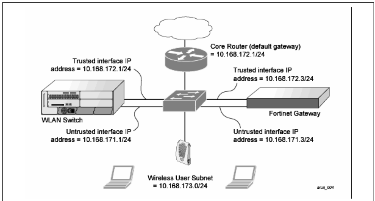
Figure 183 Example Route-Mode Topology
