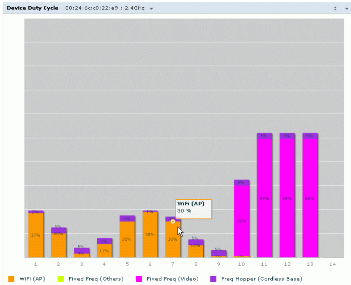
Figure 142 Device Duty Cycle
