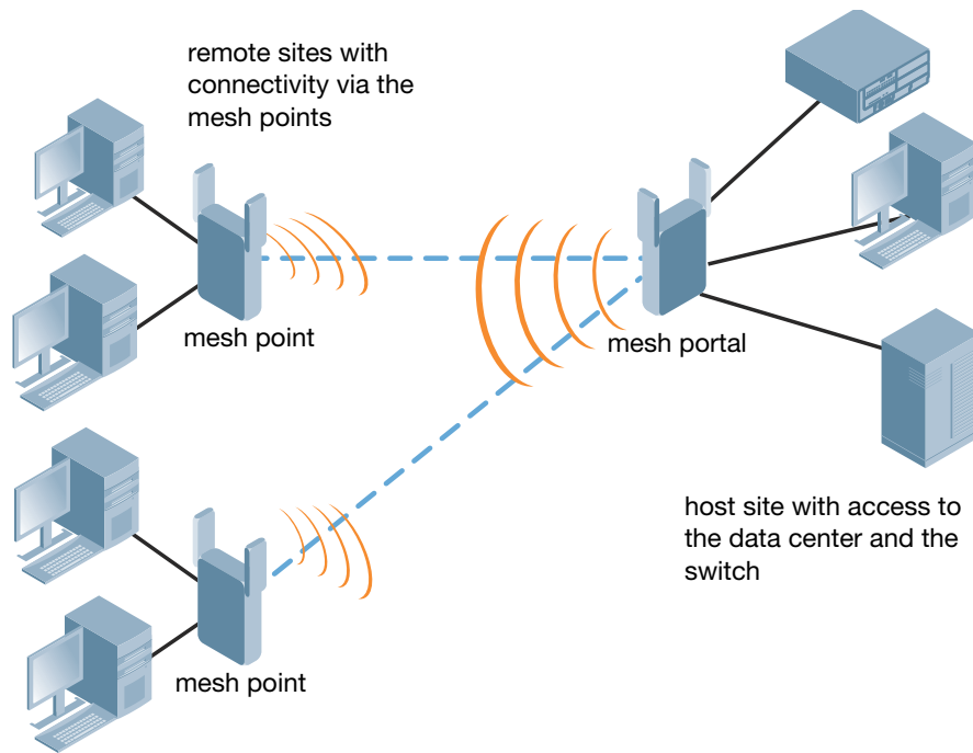
Figure 37 Sample Point-to-Multipoint Deployment
