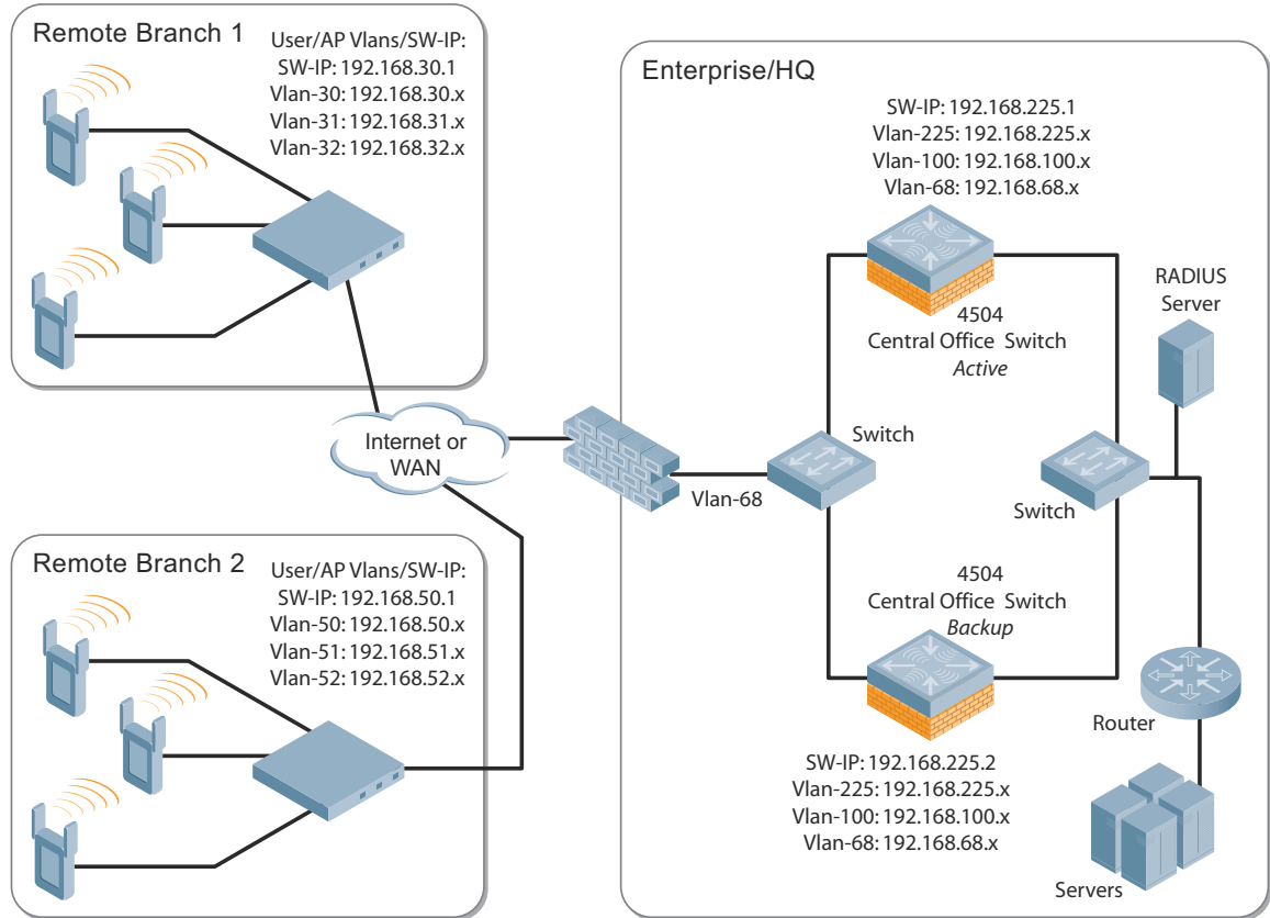
Figure 108 Sample OSPF Topology
