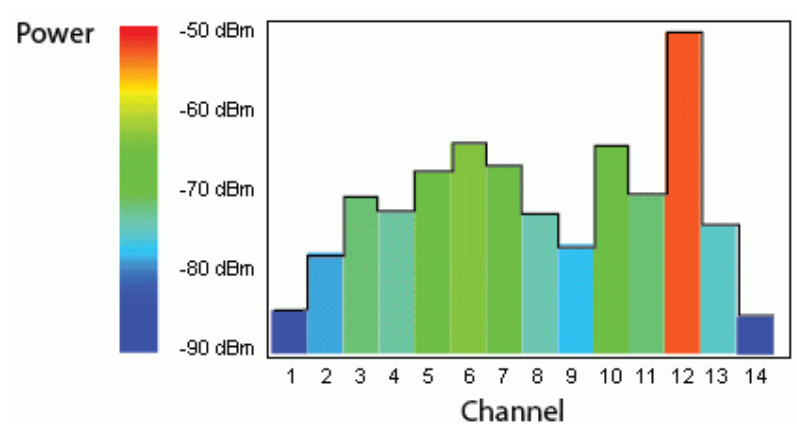
Figure 150 FFT Power Line Graph with Color
