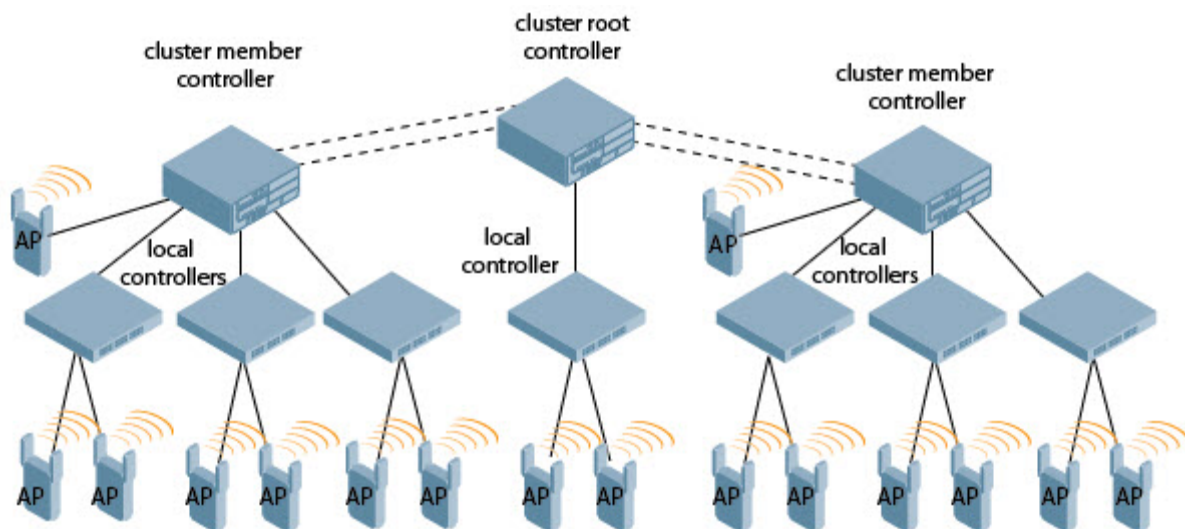
Figure 69 A Cluster of Master Switches using Control Plane Security
