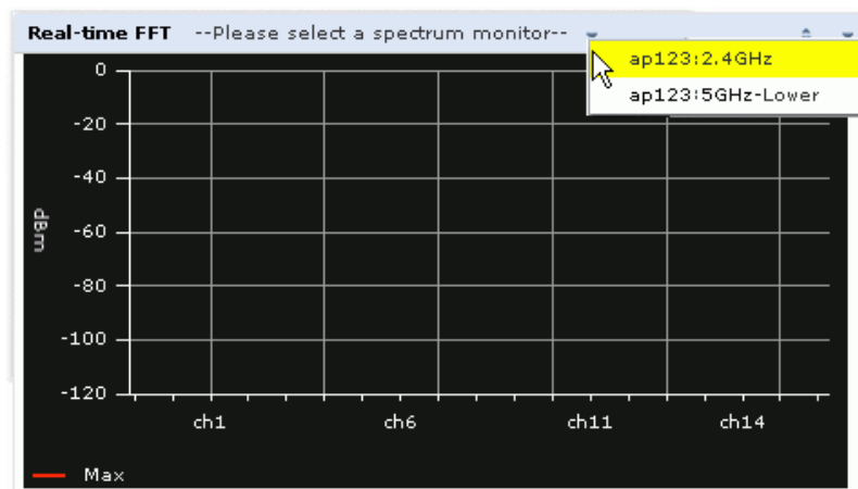
Figure 130 Selecting a Spectrum Monitor
