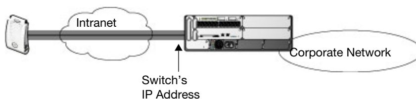
Figure 24 Remote AP with a Private Network
