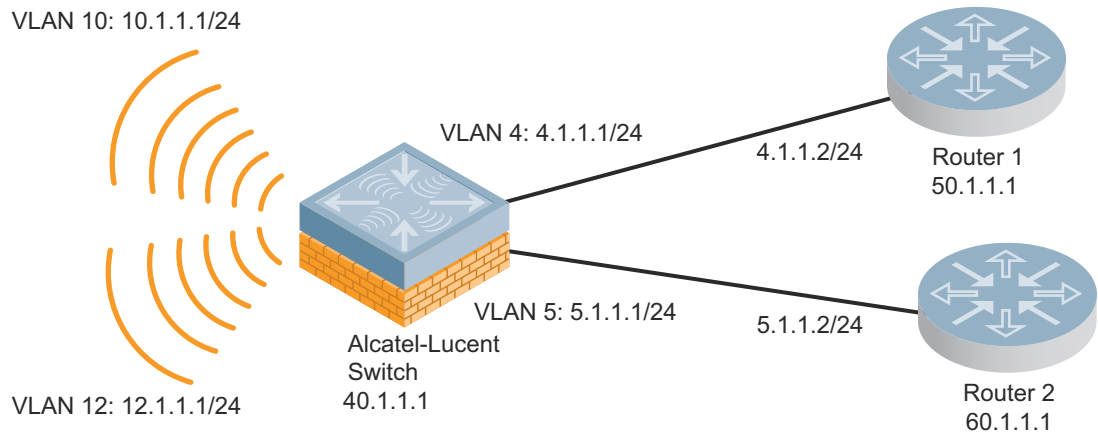
Figure 103 WLAN OSPF Topology
