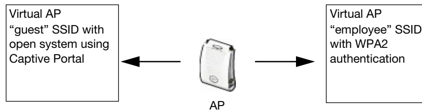
Figure 19 Virtual AP Configurations Applied to the same AP
