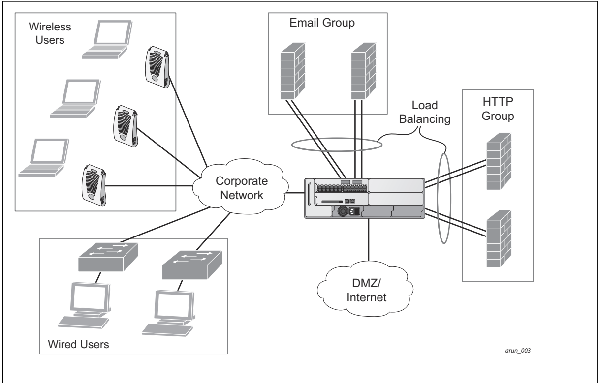
Figure 180 Load Balancing Groups
