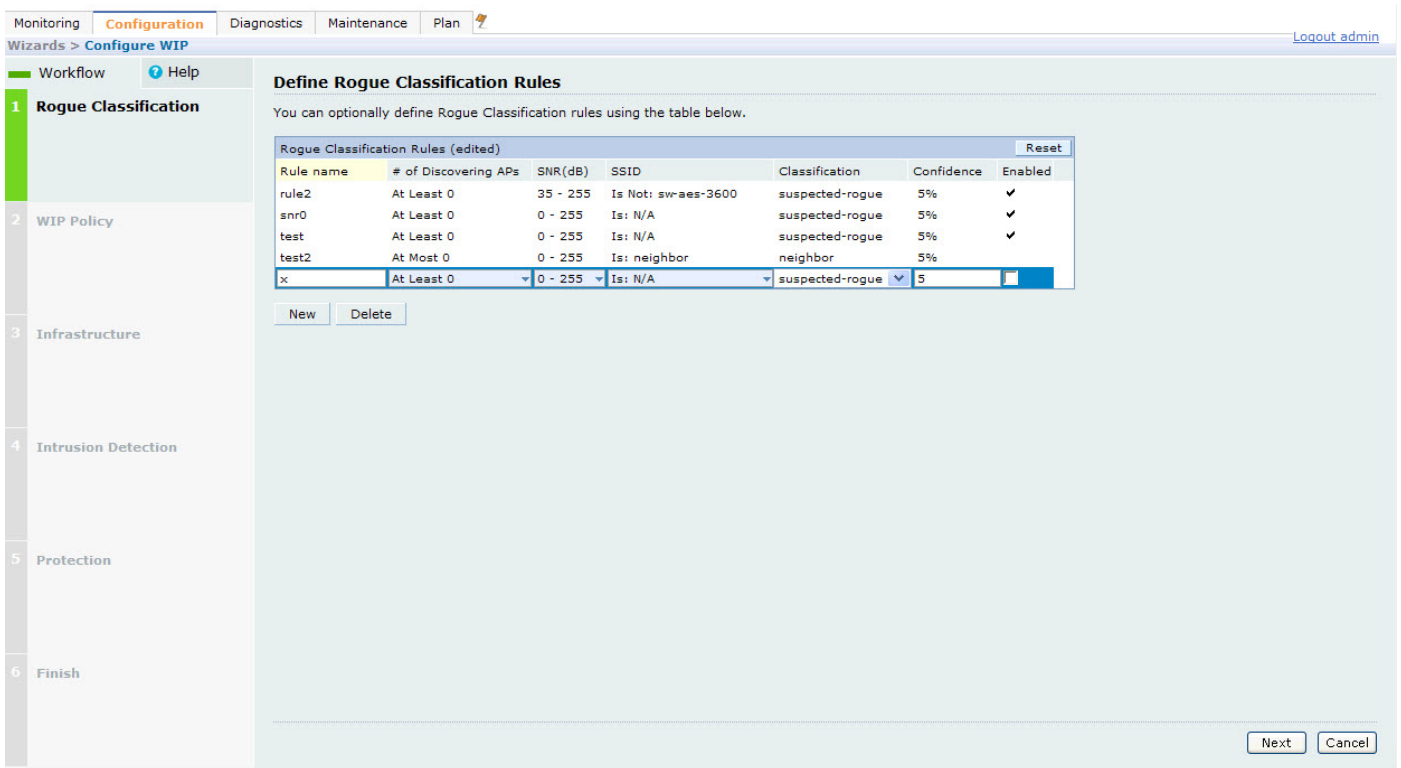
Figure 109 WIP Wizard
