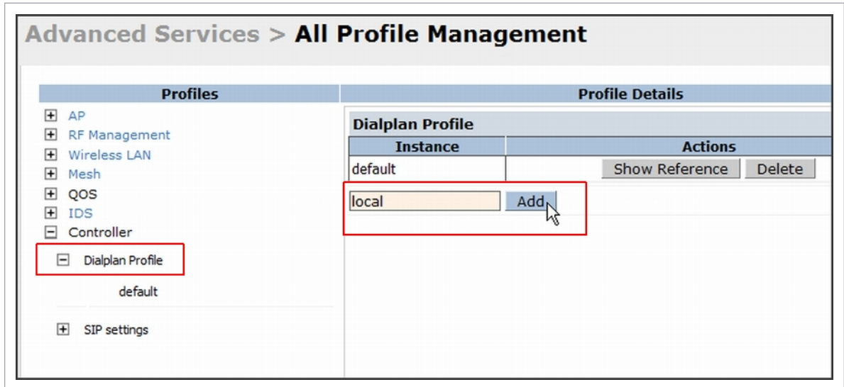
Figure 173 Dialplan Profile
