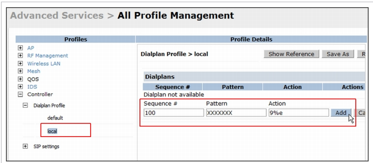
Figure 174 Dialplan Details
