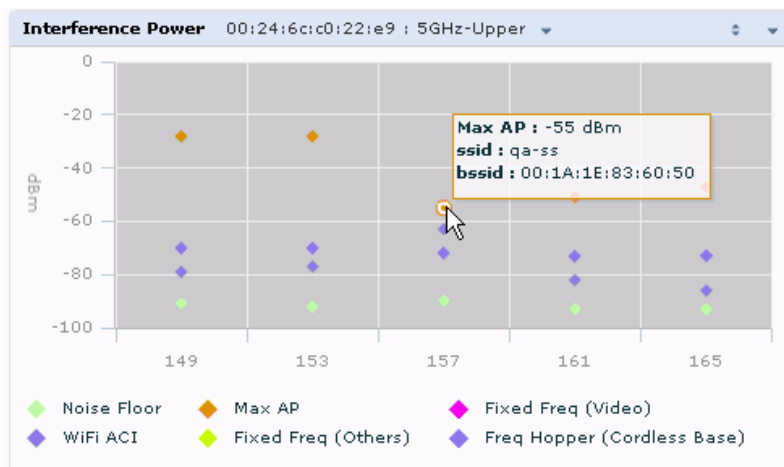
Figure 146 Interference Power
