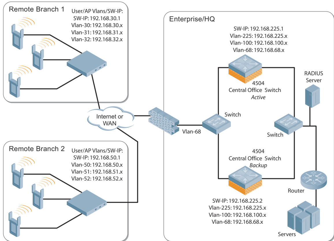
Figure 102 4306 Series Sample Topology
