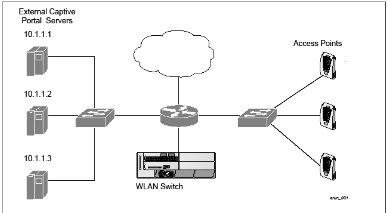
Figure 184 Example NAT-Mode Topology
