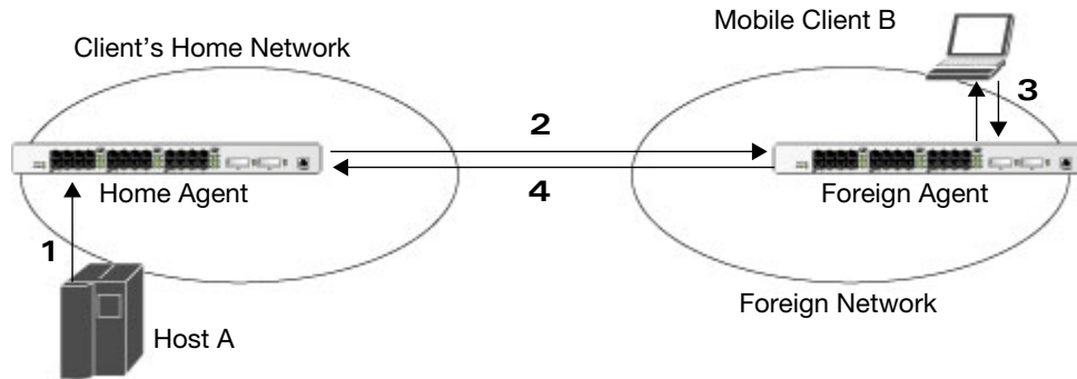
Figure 73 Routing of Traffic to Mobile Client within Mobility Domain
