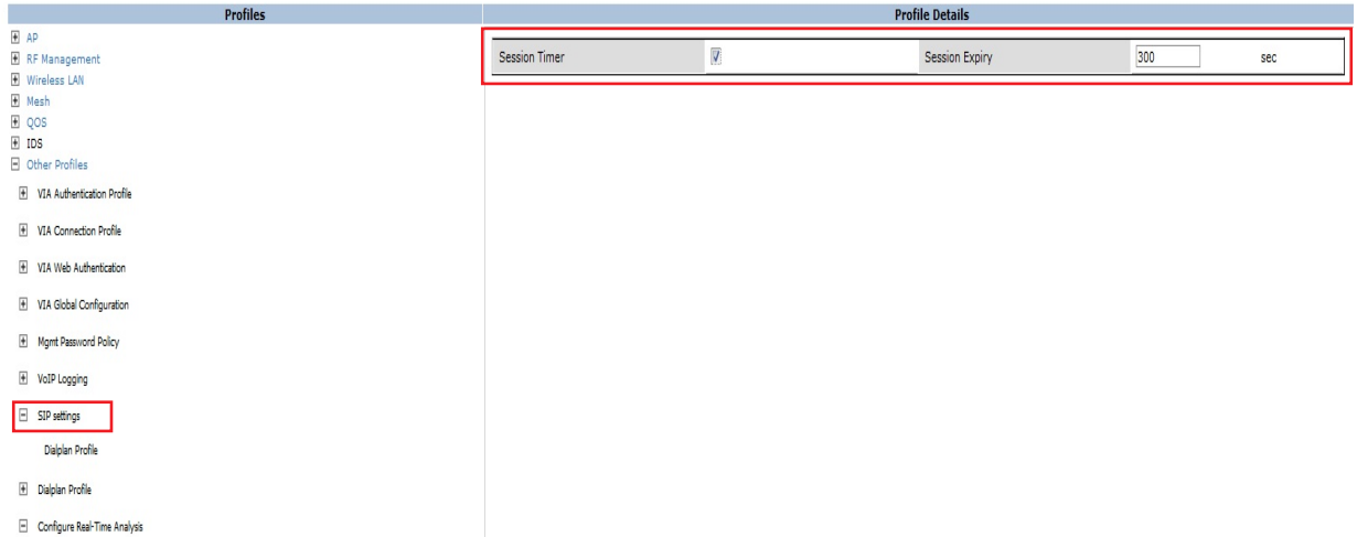
Figure 169 Enabling SIP Session Timer
