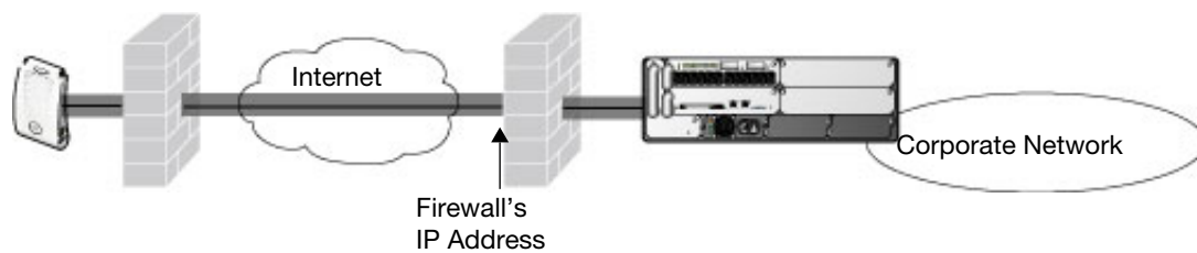
Figure 26 Remote AP with Switch Behind Firewall
