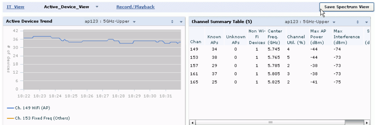
Figure 133 Save a Spectrum Analysis Dashboard Layout
