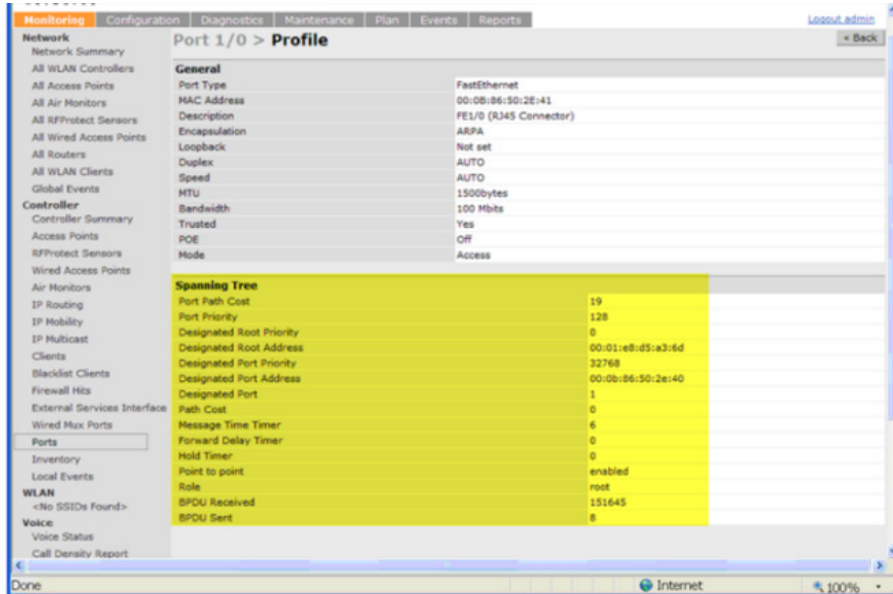
Figure 79 Monitoring RSTP
