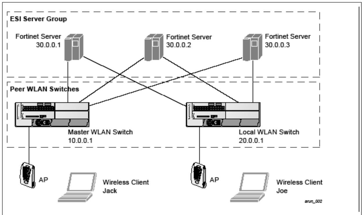
Figure 182 Peer Switches
