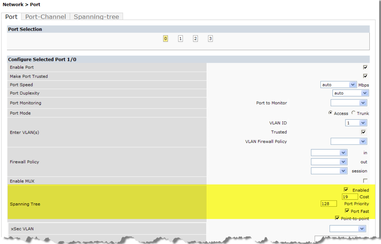
Figure 78 Configuring RSTP
