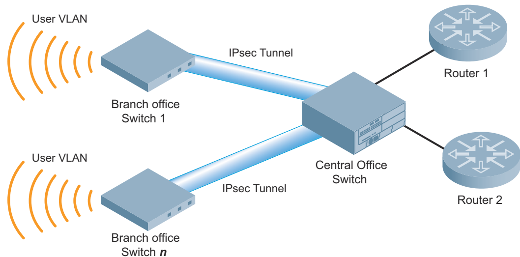
Figure 104 Branch Office OSPF Topology
