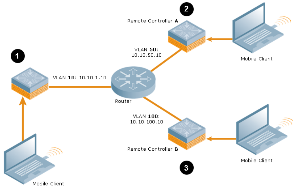
Figure 76 Inter-switch Mobility
