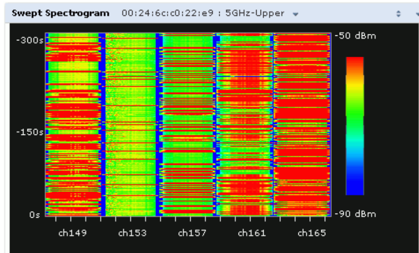
Figure 152 Swept Spectrogram
